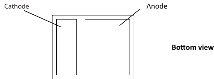
Figure 2. Pad configuration.
