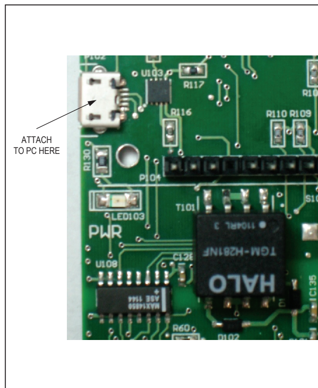
Figure 4. MAX14921 EV Kit Attachment
