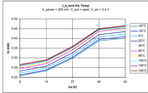
Is vers Vs_Temp_200mV_Voutopen.vsd
