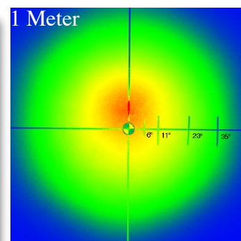
PL50040 (40°) Spectro Metric Analysis
